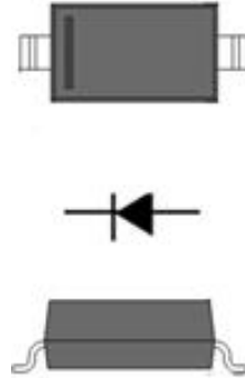
SOD-323
